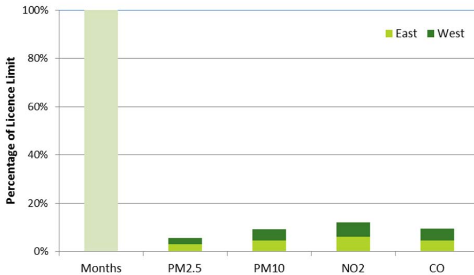
Figure 20: Ventilation Stack Emissions as Percentage of Licence Limit (1/07/2013 - 30/06/2015)
