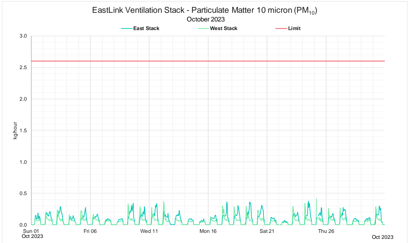
Figure 6: Monthly 1-hour mass rate PM 10
