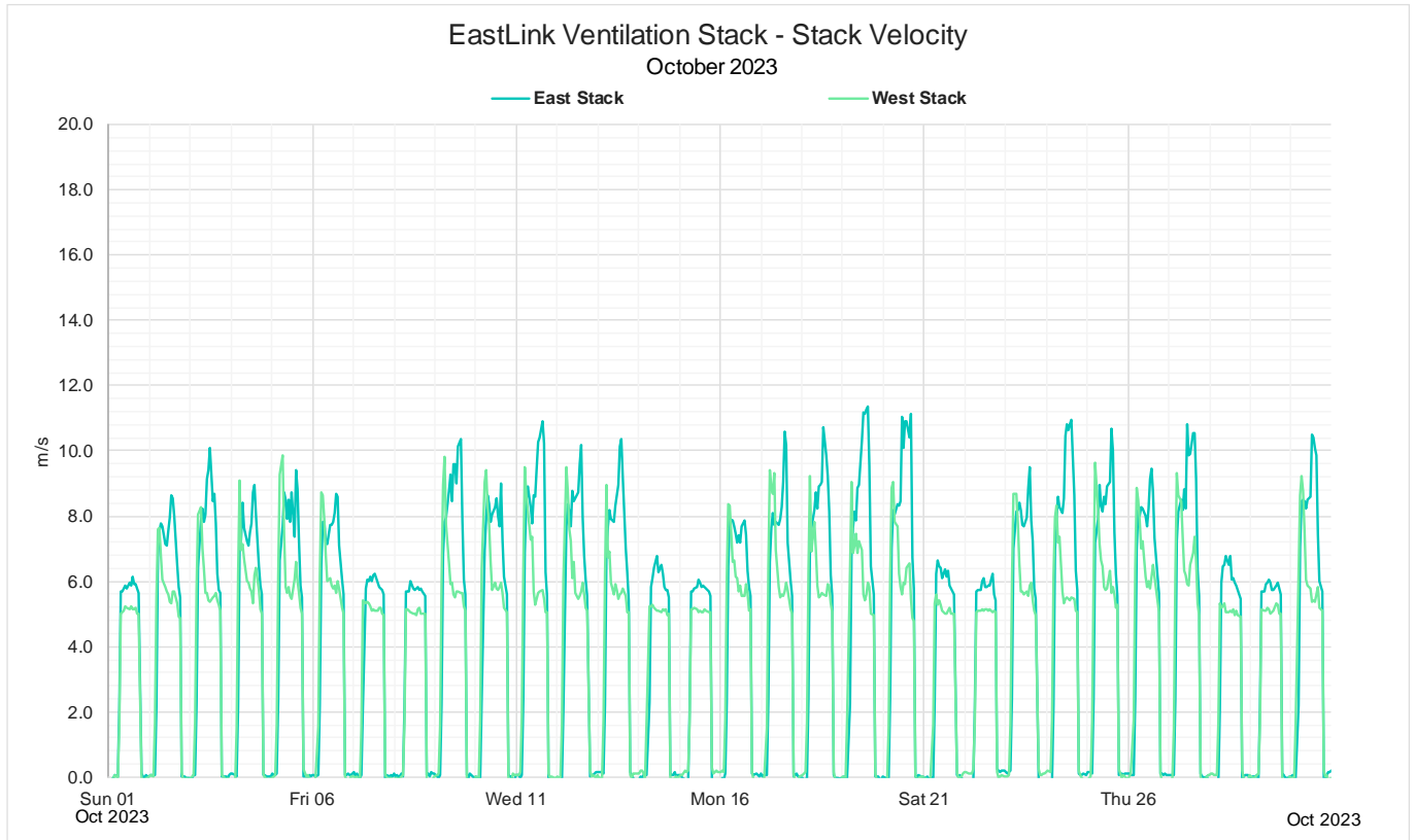
Figure 7: Monthly 1-hour average stack velocity
