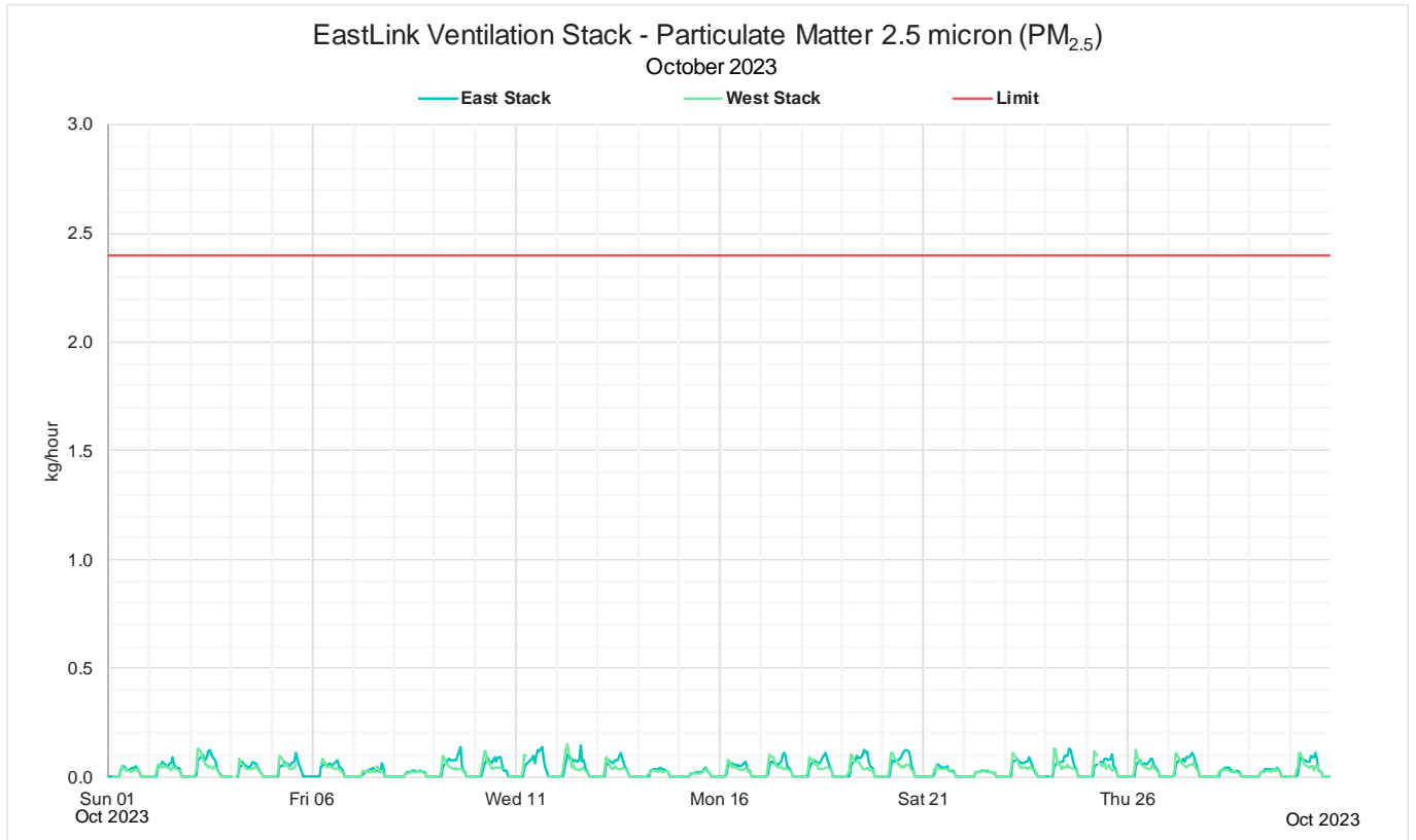
Figure 5: Monthly 1-hour mass rate PM 2.5
