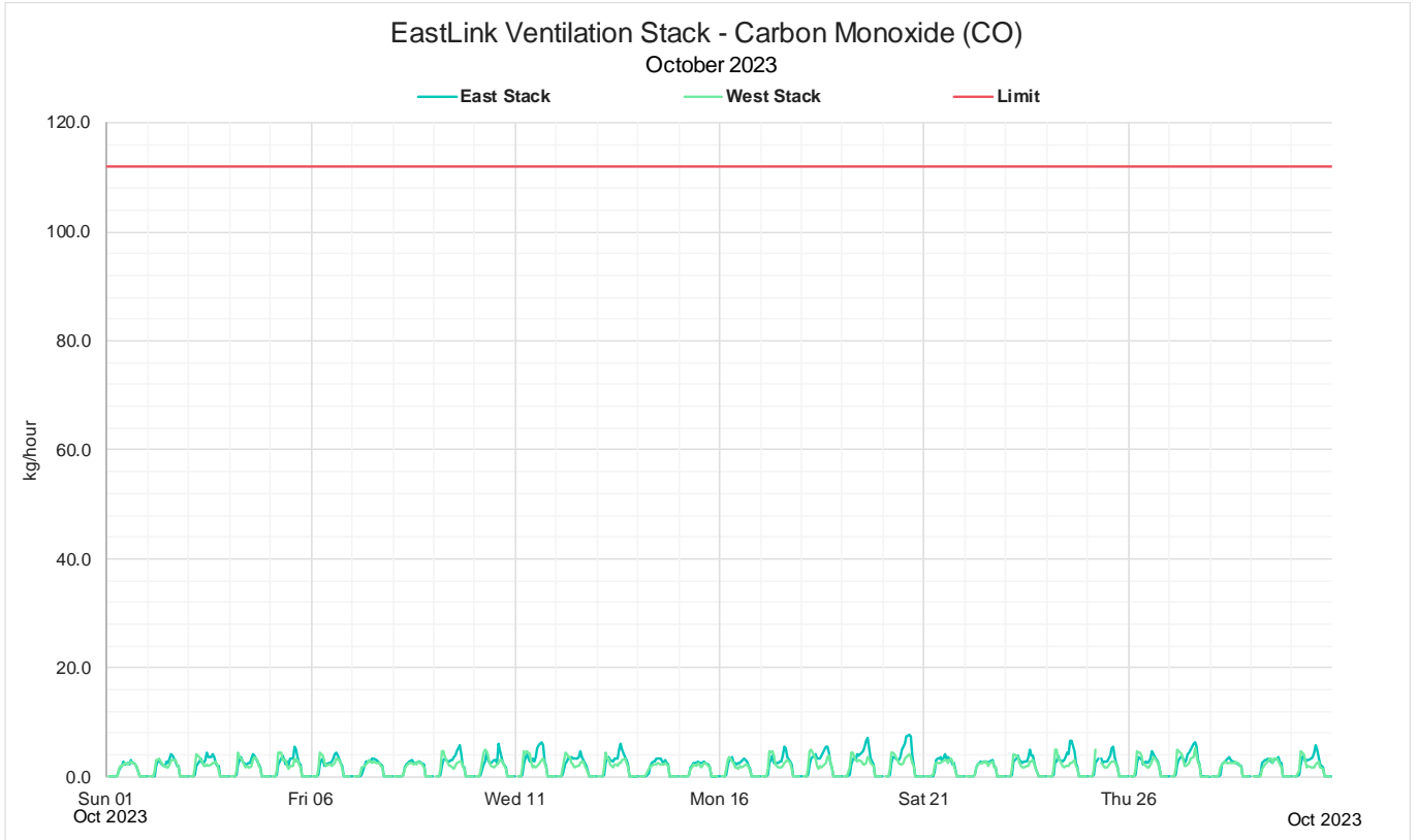
Figure 4: Monthly 1-hour mass rate CO
