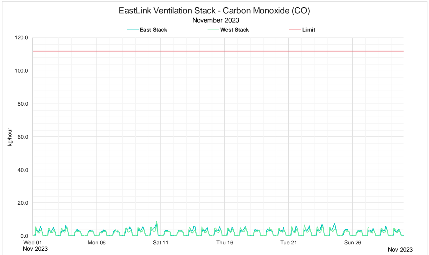
Figure 11: Monthly 1-hour mass rate CO
