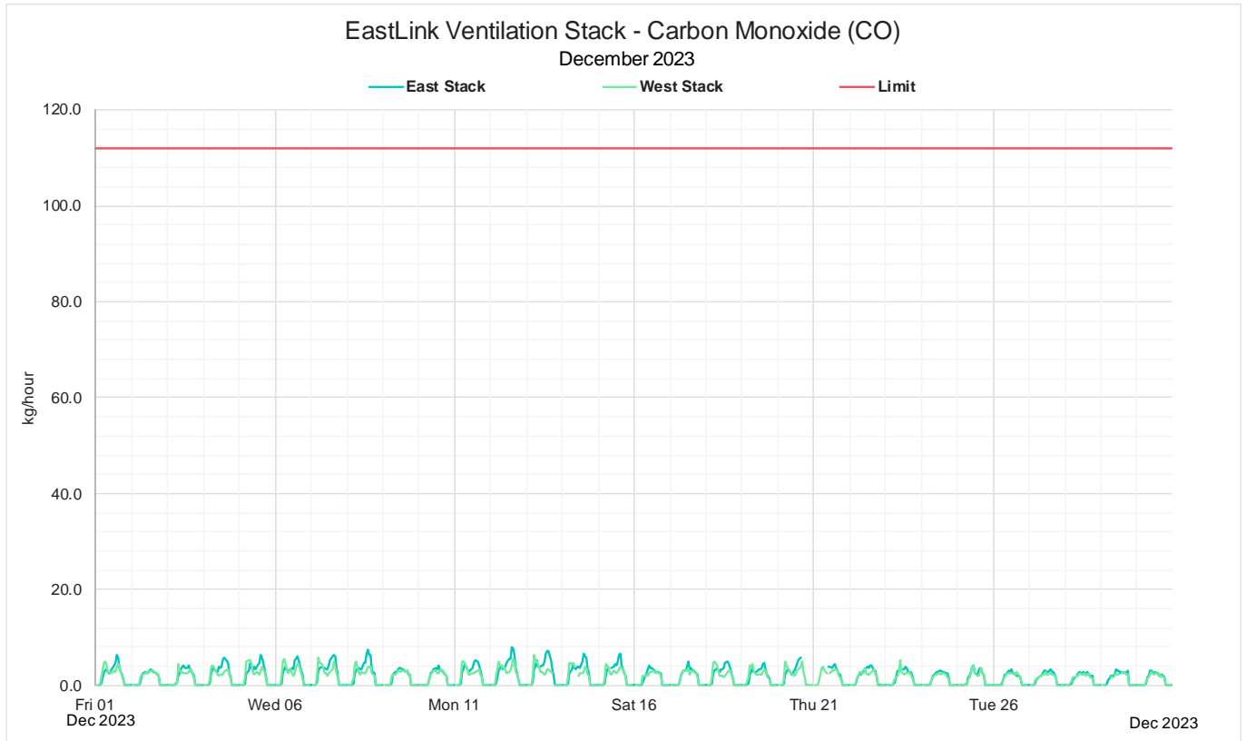
Figure 18: Monthly 1-hour mass rate CO
