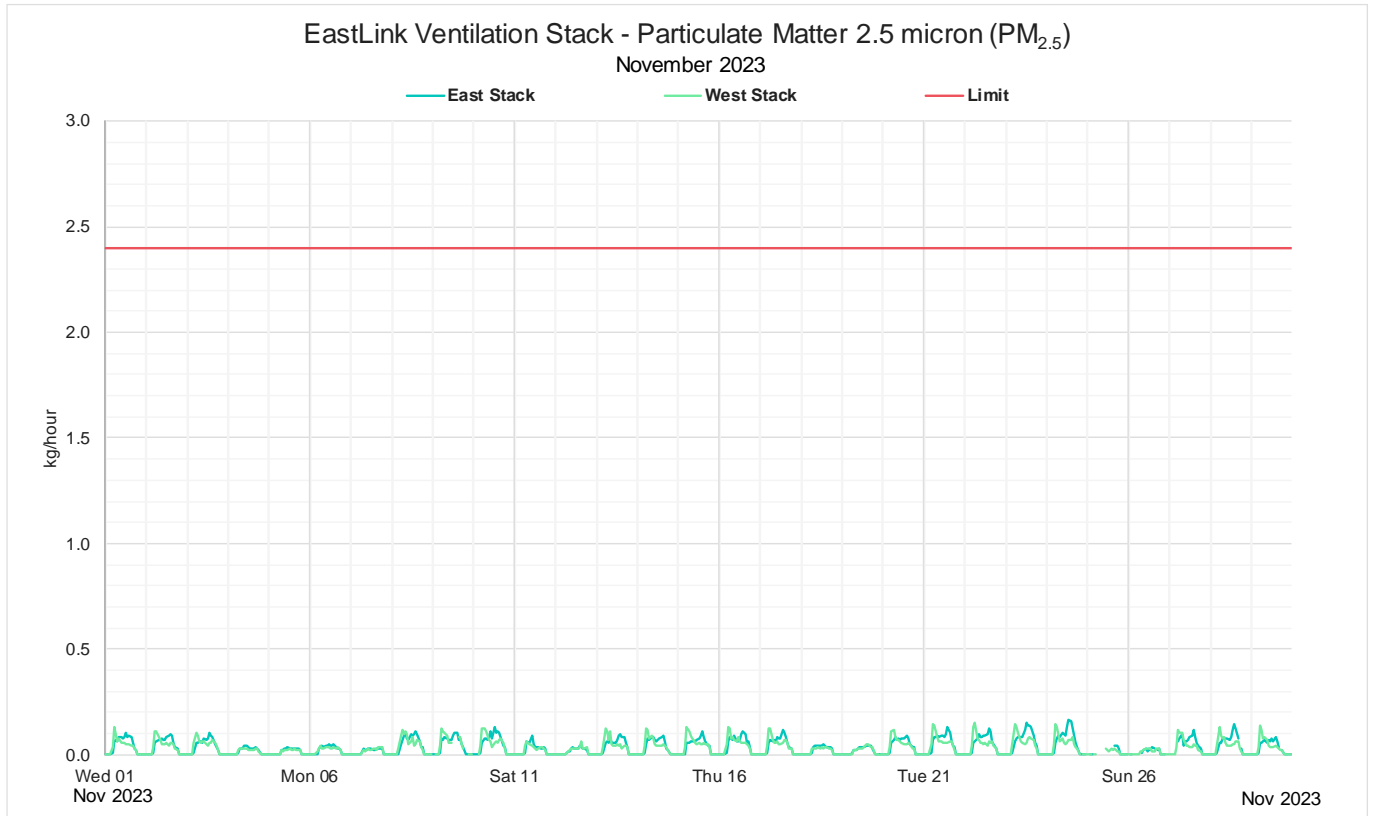
Figure 12: Monthly 1-hour mass rate PM 2.5
