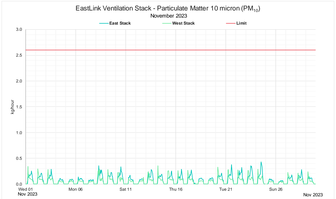
Figure 13: Monthly 1-hour mass rate PM 10
