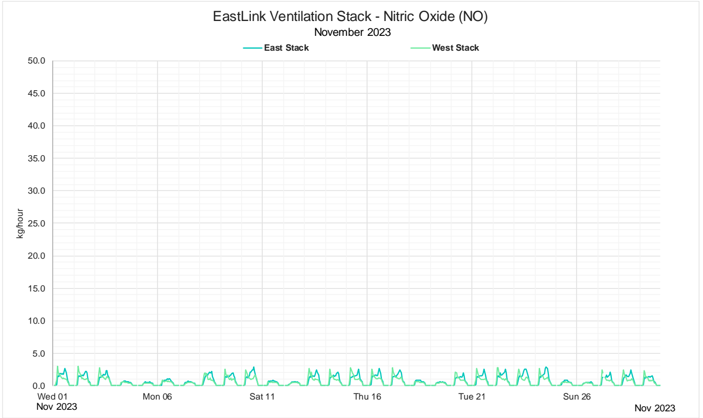
Figure 10: Monthly 1-hour mass rate NO
