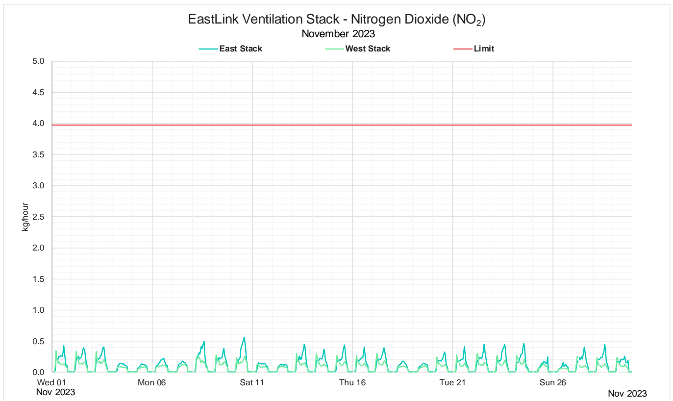
Figure 9: Monthly 1-hour mass rate NO 2
