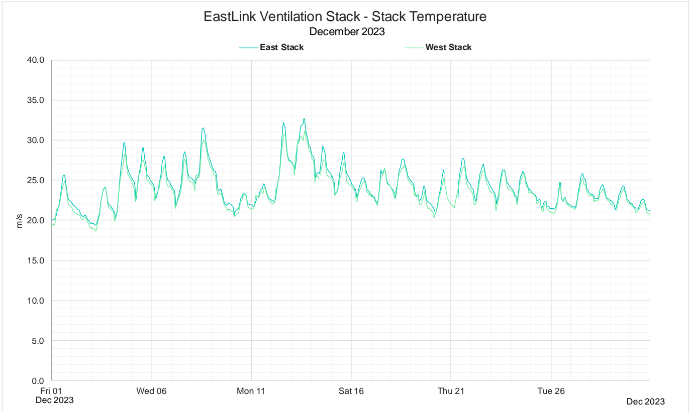
Figure 22: Monthly 1-hour average stack temperature
