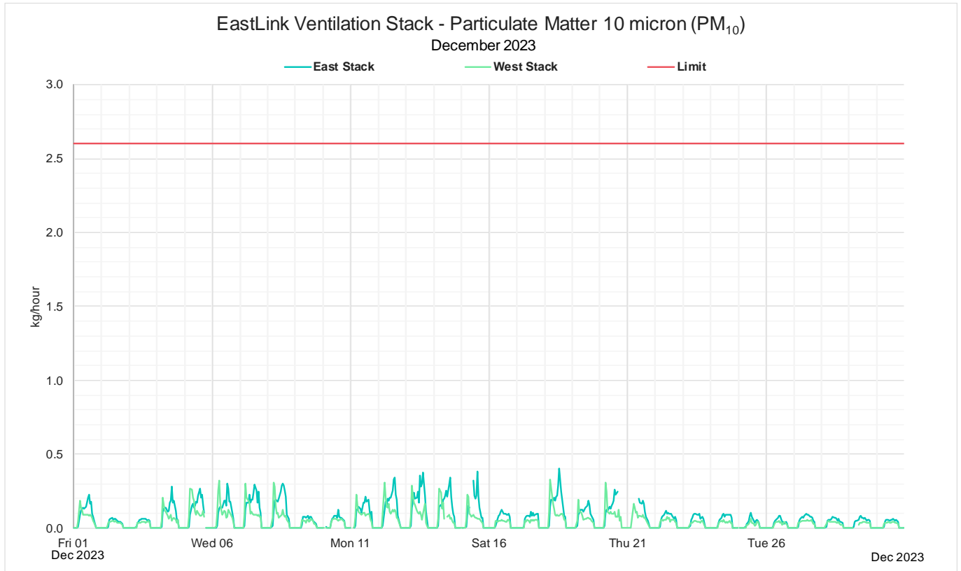
Figure 20: Monthly 1-hour mass rate PM 10
