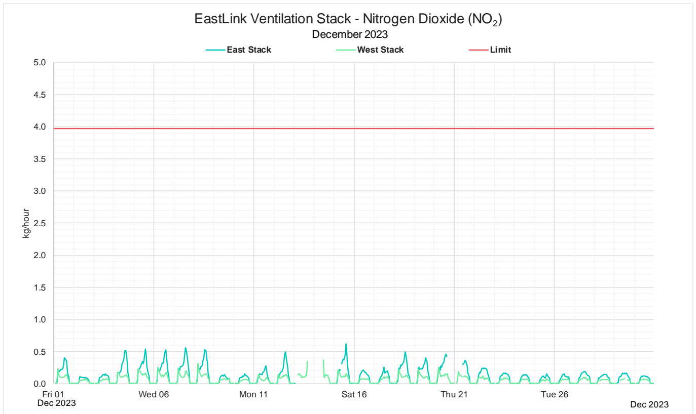
Figure 16: Monthly 1-hour mass rate NO 2
