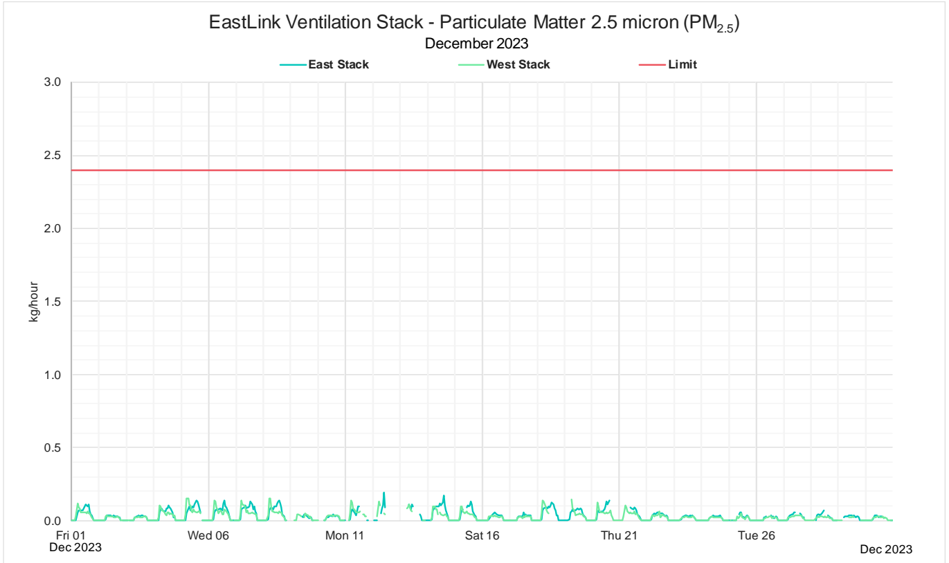
Figure 19: Monthly 1-hour mass rate PM 2.5
