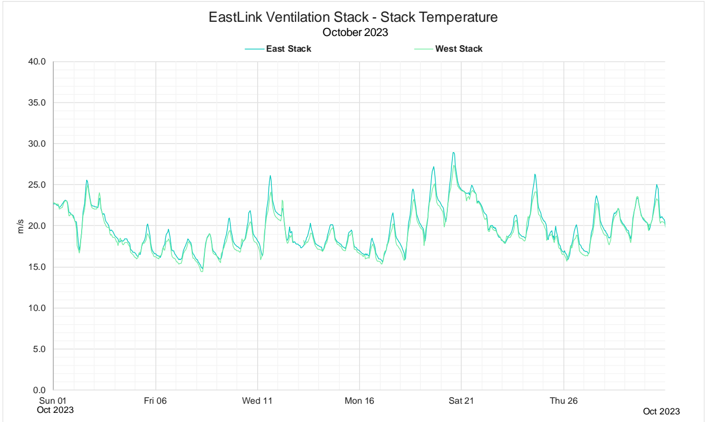
Figure 8: Monthly 1-hour average stack temperature
