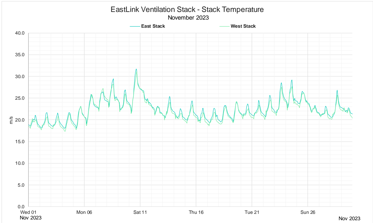
Figure 15: Monthly 1-hour average stack temperature
