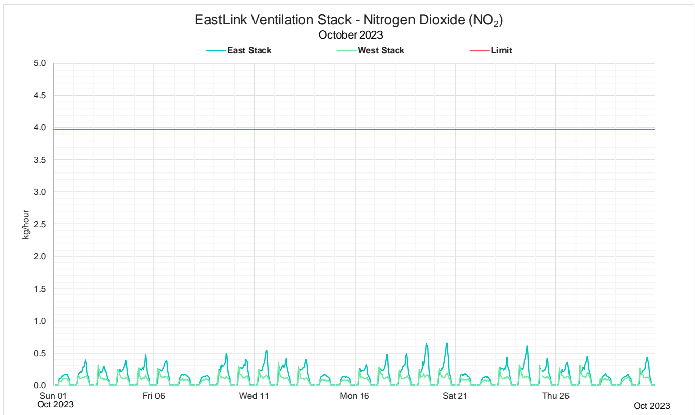
Figure 2: Monthly 1-hour mass rate NO 2
