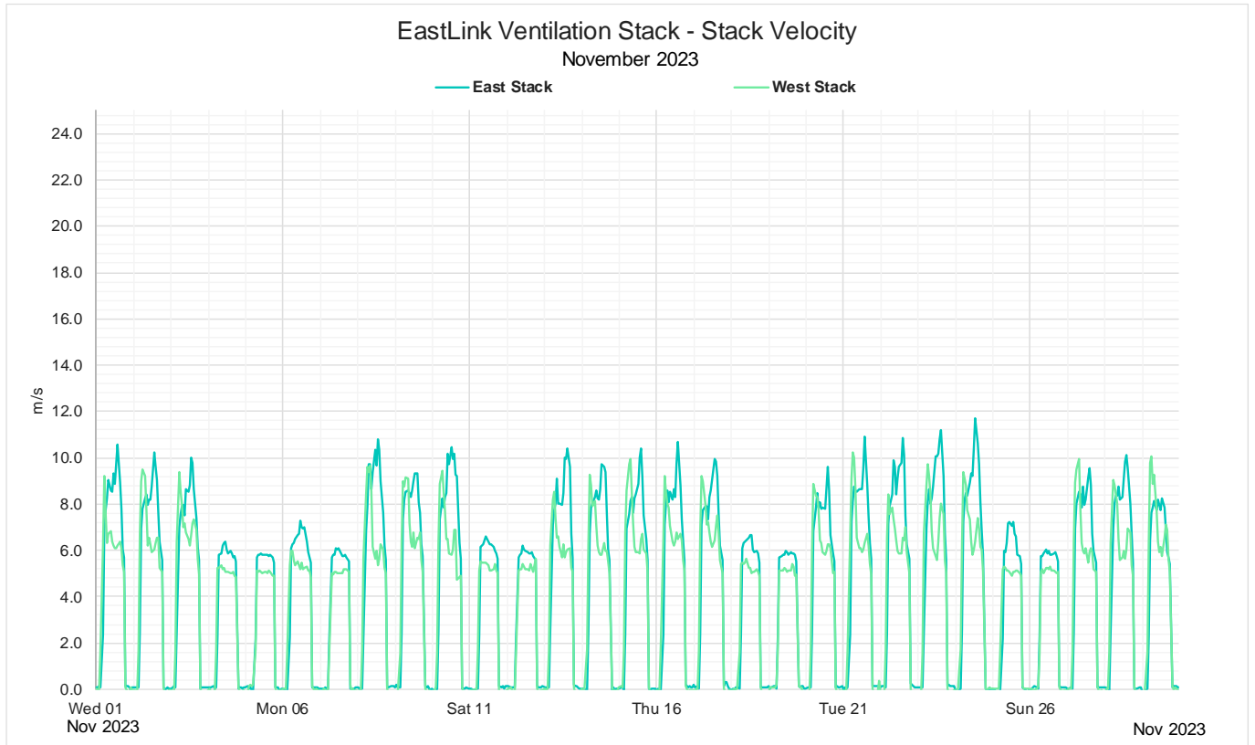
Figure 14: Monthly 1-hour average stack velocity
