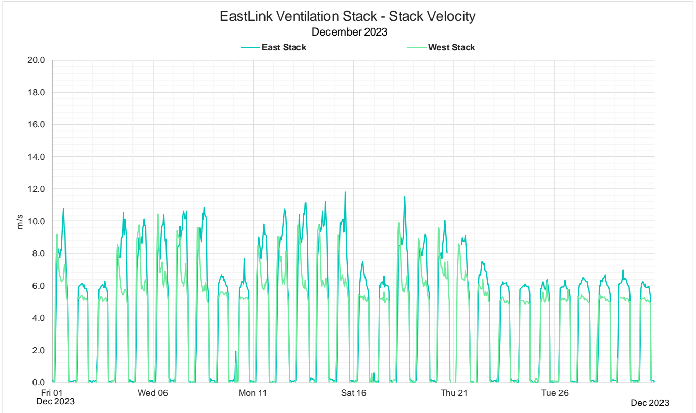
Figure 21: Monthly 1-hour average stack velocity
